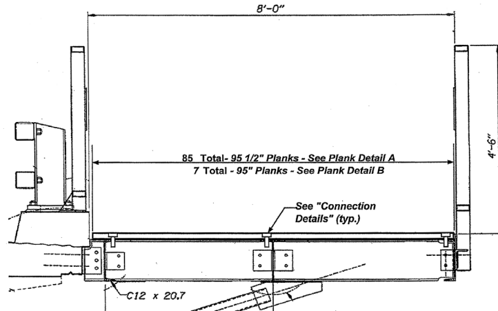
TYPICAL SECTION
